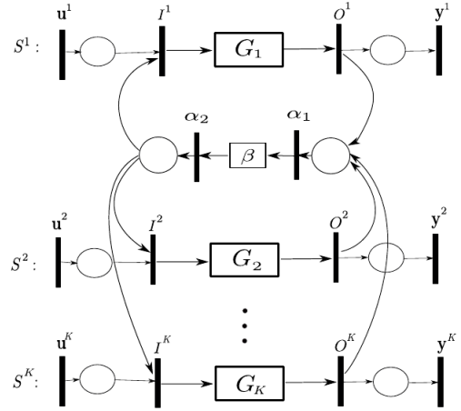
Fig. 2. Resource-sharing TEGs.
