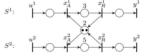
Fig. 4. Two TEGs sharing a resource with capacity 2.
