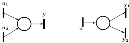
Fig. 3. A join and a fork structure.
