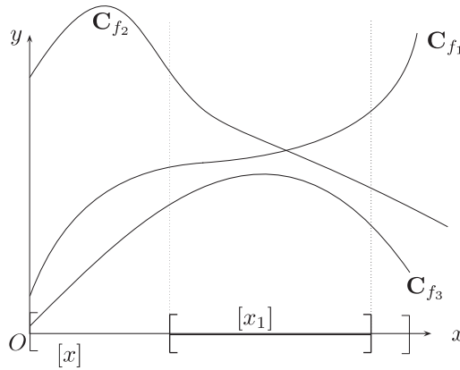
Figure 4. Graphs of functions f_1, f_2 and f_3 .
