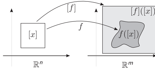
Figure 3. Inclusion function [f] of a function f .
