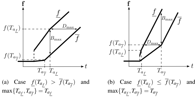
Fig. 11 Maximal uncertainty \Sigma_{\mathbf{f}} = \{ D_{\max}, B_{\max} \} of a container \mathbf{f} \in \mathbf{F}
