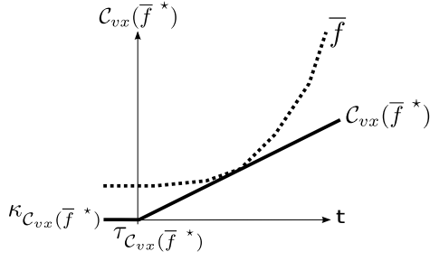
Fig. 12 Upper bound \bar{f} of a container \mathbf{f} \in \mathbf{F} and the convex approximation of its subadditive closure \mathcal{C}_{vx}(\bar{f}^*)
