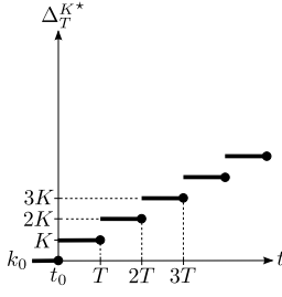
Fig. 3 Subadditive closure of an elementary function: \Delta_T^{K*} \in \mathcal{F}_{cp}
