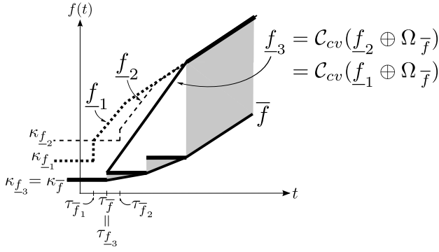
Fig. 10 Canonical representation [\underline{f}_3, \bar{f}]_{\mathcal{L}} of the identical containers [\underline{f}_1, \bar{f}]_{\mathcal{L}} and [\underline{f}_2, \bar{f}]_{\mathcal{L}}
