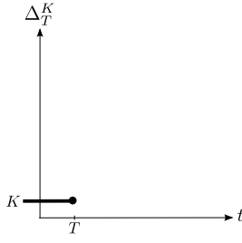
Fig. 1 An elementary function \Delta_T^K
