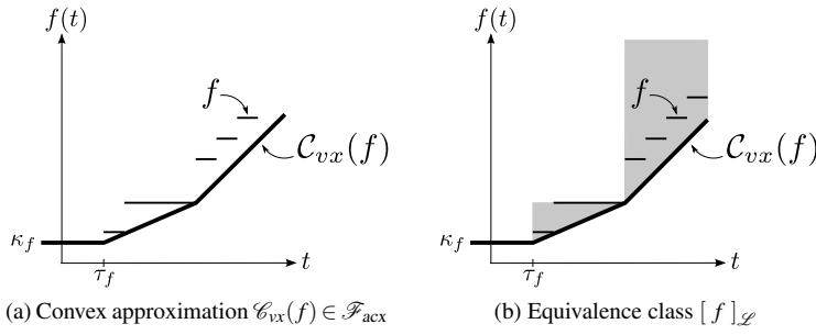
Fig. 7 Convex approximation of f \in \mathcal{F}_{cp} and its equivalence class modulo the Legendre-Fenchel transform \mathcal{L}
