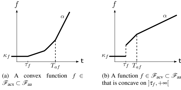
Fig. 5 Examples of ultimately affine functions
