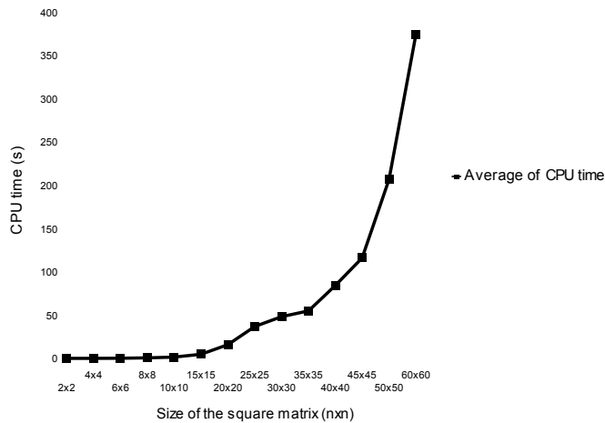
Fig. 16 CPU time of the computation of A^{[*]} , depending on the size of A
