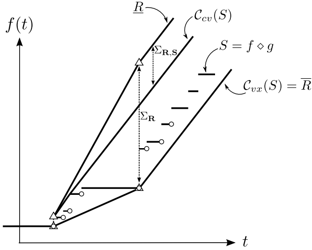
Fig. 14 Pessimism and memory consumption between the approximated computations \mathbf{R} and the exact ones S \in \mathbf{S}
