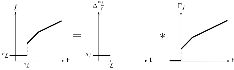
Fig. 6 Factorization of a concave function f \in \mathcal{F}_{acv} : f = \Delta_{\tau_f}^{\kappa_f} * \Gamma_f
