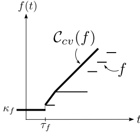
Fig. 8 Concave approximation of f \in \mathcal{F}_{cp} : \mathcal{C}_{cv}(f) \in \mathcal{F}_{acv}
