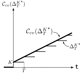
Fig. 13 Concave approximation of the subadditive closure of an elementary function: \mathcal{C}_{cv}(\Delta_T^{K*}) \in \mathcal{F}_{acv} .
