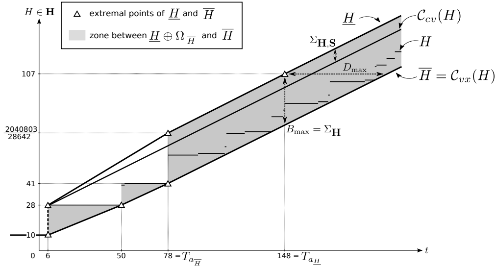
Fig. 15 Transfer matrix H^{1 \times 1} \in \mathcal{F}_{cp} and its container \mathbf{H} = [\underline{H}, \overline{H}] \in \mathbf{F}
