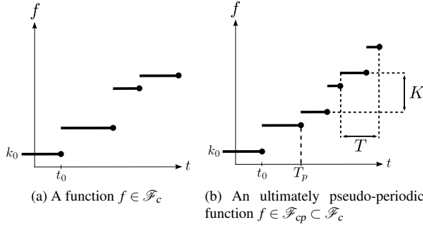
Fig. 2 Examples of piecewise constant functions
